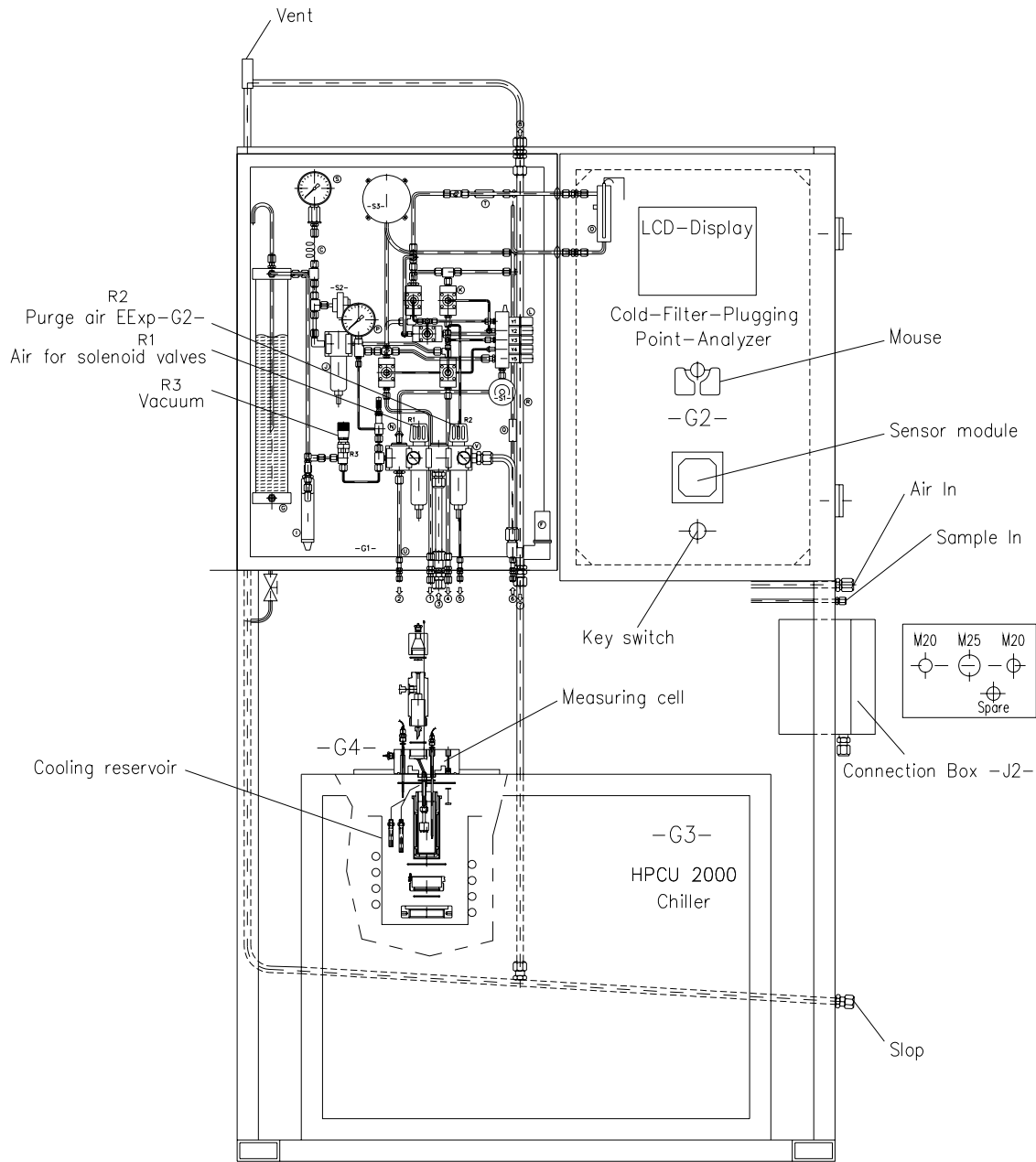
Figure 3: Exemplary layout drawing of the CFPP
